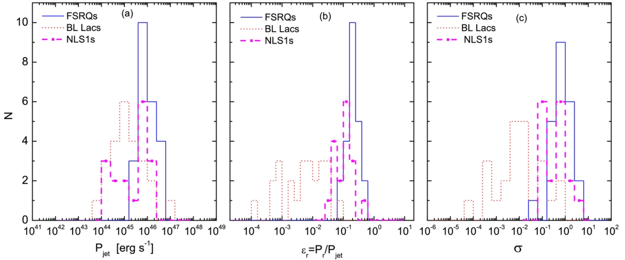
Figure 4. from Jet Properties of GeV-selected Radio-loud Narrow-line Seyfert 1 Galaxies and Possible Connection to Their Disk and Corona Sun et al. 2015 ApJ 798 43 doi:10.1088/0004-637X/798/1/43 https://dx.doi.org/10.1088/0004-637X/798/1/43 © 2015. The American Astronomical Society. All rights reserved.
