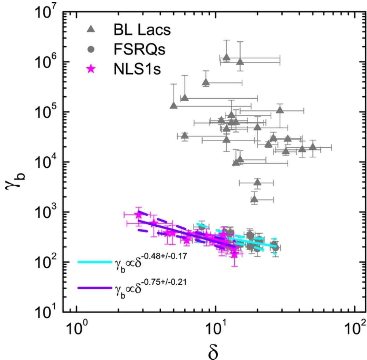
Figure 3. from Jet Properties of GeV-selected Radio-loud Narrow-line Seyfert 1 Galaxies and Possible Connection to Their Disk and Corona Sun et al. 2015 ApJ 798 43 doi:10.1088/0004-637X/798/1/43 https://dx.doi.org/10.1088/0004-637X/798/1/43 © 2015. The American Astronomical Society. All rights reserved.
