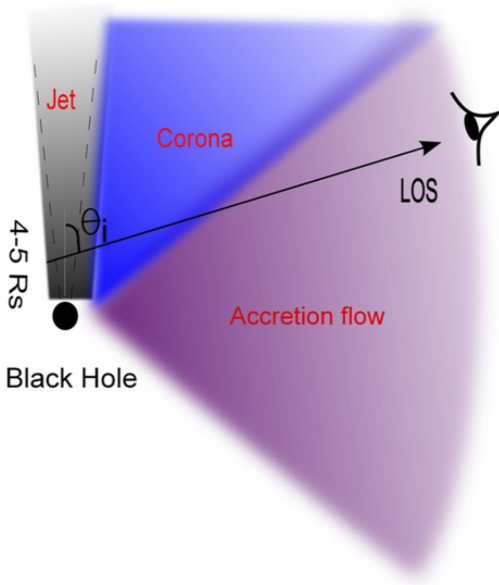
Figure 2. from Confronting the Jet Model of Sgr A* with the Faraday Rotation Measure Observations Li, Yuan, & Wang 2015 ApJ 798 22 doi:10.1088/0004-637X/798/1/22 https://dx.doi.org/10.1088/0004-637X/798/1/22 © 2015. The American Astronomical Society. All rights reserved.
