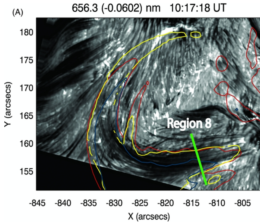
Figure 9. from Unresolved Fine-scale Structure in Solar Coronal Loop-tops Scullion et al. 2014 ApJ 797 36 doi:10.1088/0004-637X/797/1/36 https://dx.doi.org/10.1088/0004-637X/797/1/36 © 2014. The American Astronomical Society. All rights reserved.
