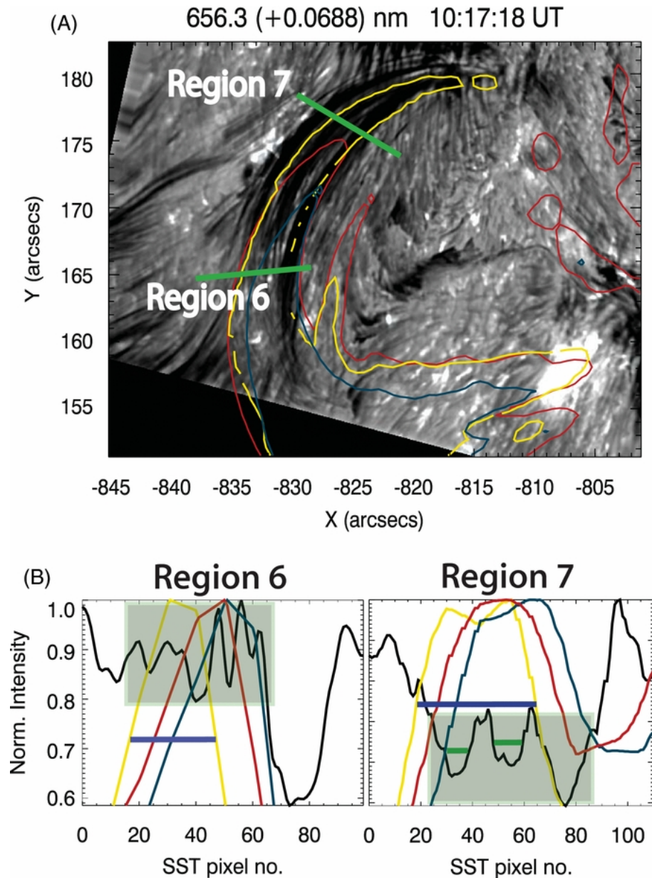
Figure 8. from Unresolved Fine-scale Structure in Solar Coronal Loop-tops Scullion et al. 2014 ApJ 797 36 doi:10.1088/0004-637X/797/1/36 https://dx.doi.org/10.1088/0004-637X/797/1/36 © 2014. The American Astronomical Society. All rights reserved.
