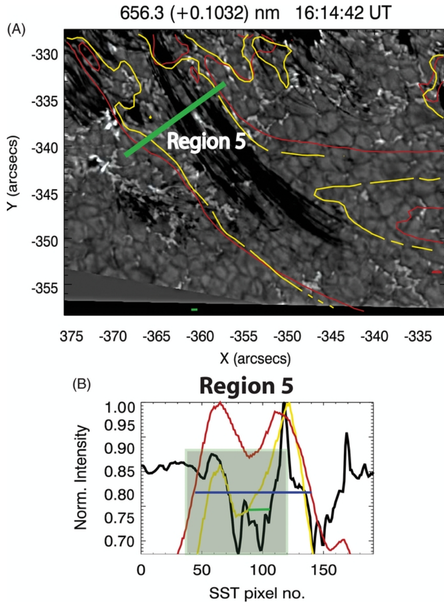
Figure 7. from Unresolved Fine-scale Structure in Solar Coronal Loop-tops Scullion et al. 2014 ApJ 797 36 doi:10.1088/0004-637X/797/1/36 https://dx.doi.org/10.1088/0004-637X/797/1/36 © 2014. The American Astronomical Society. All rights reserved.
