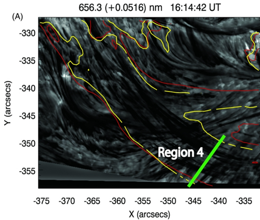
Figure 6. from Unresolved Fine-scale Structure in Solar Coronal Loop-tops Scullion et al. 2014 ApJ 797 36 doi:10.1088/0004-637X/797/1/36 https://dx.doi.org/10.1088/0004-637X/797/1/36 © 2014. The American Astronomical Society. All rights reserved.
