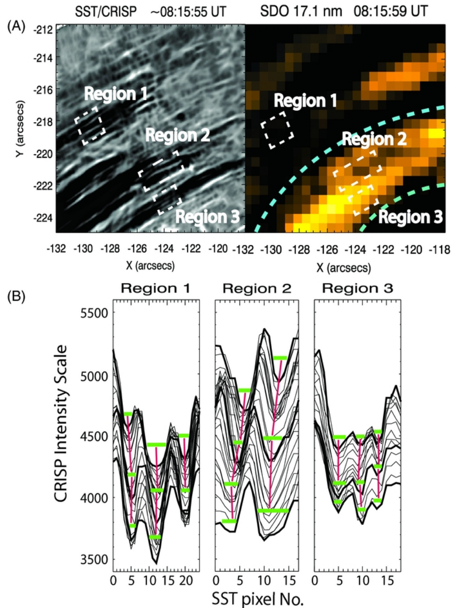
Figure 5. from Unresolved Fine-scale Structure in Solar Coronal Loop-tops Scullion et al. 2014 ApJ 797 36 doi:10.1088/0004-637X/797/1/36 https://dx.doi.org/10.1088/0004-637X/797/1/36
