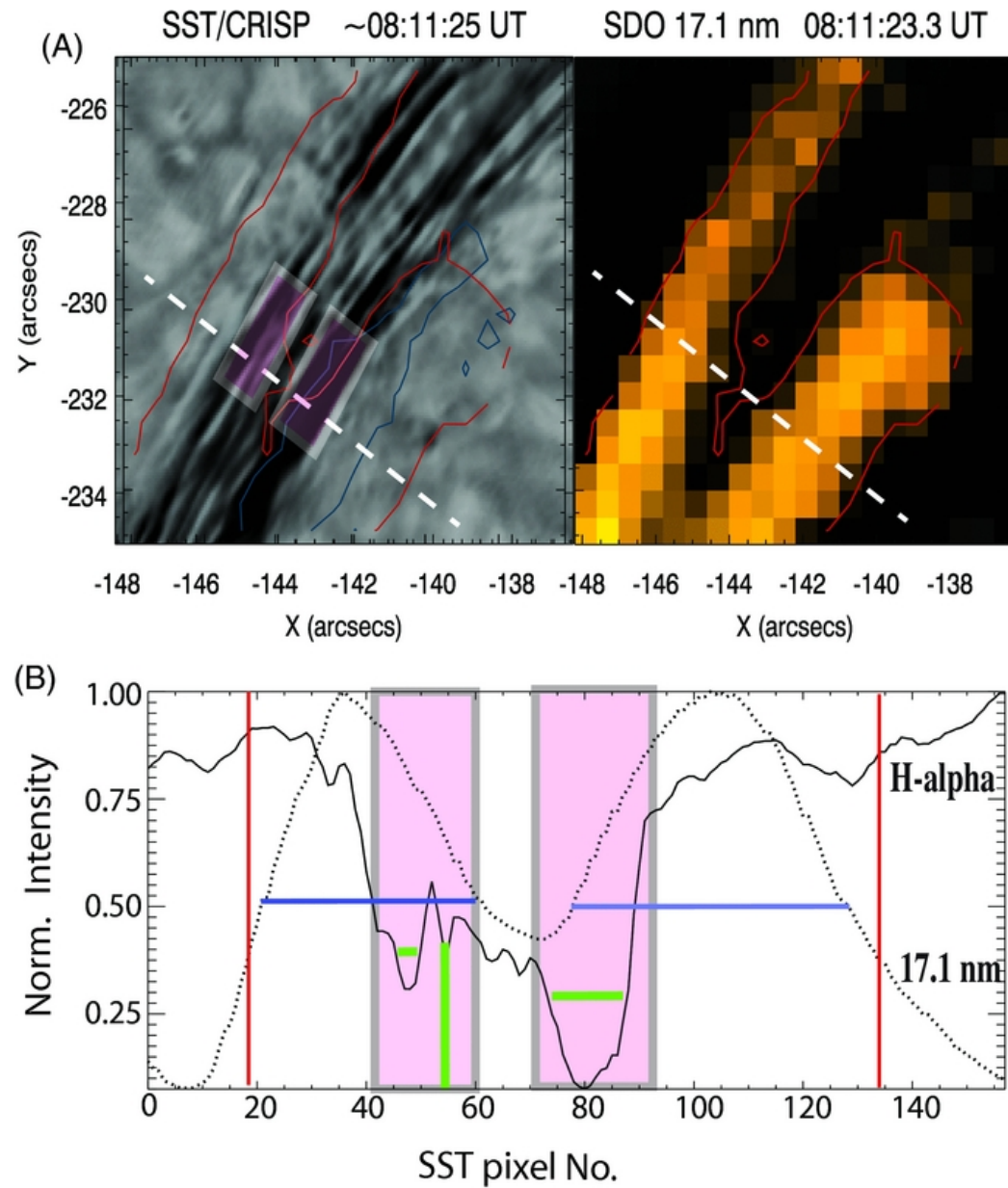
Figure 4. from Unresolved Fine-scale Structure in Solar Coronal Loop-tops Scullion et al. 2014 ApJ 797 36 doi:10.1088/0004-637X/797/1/36 https://dx.doi.org/10.1088/0004-637X/797/1/36 © 2014. The American Astronomical Society. All rights reserved.
