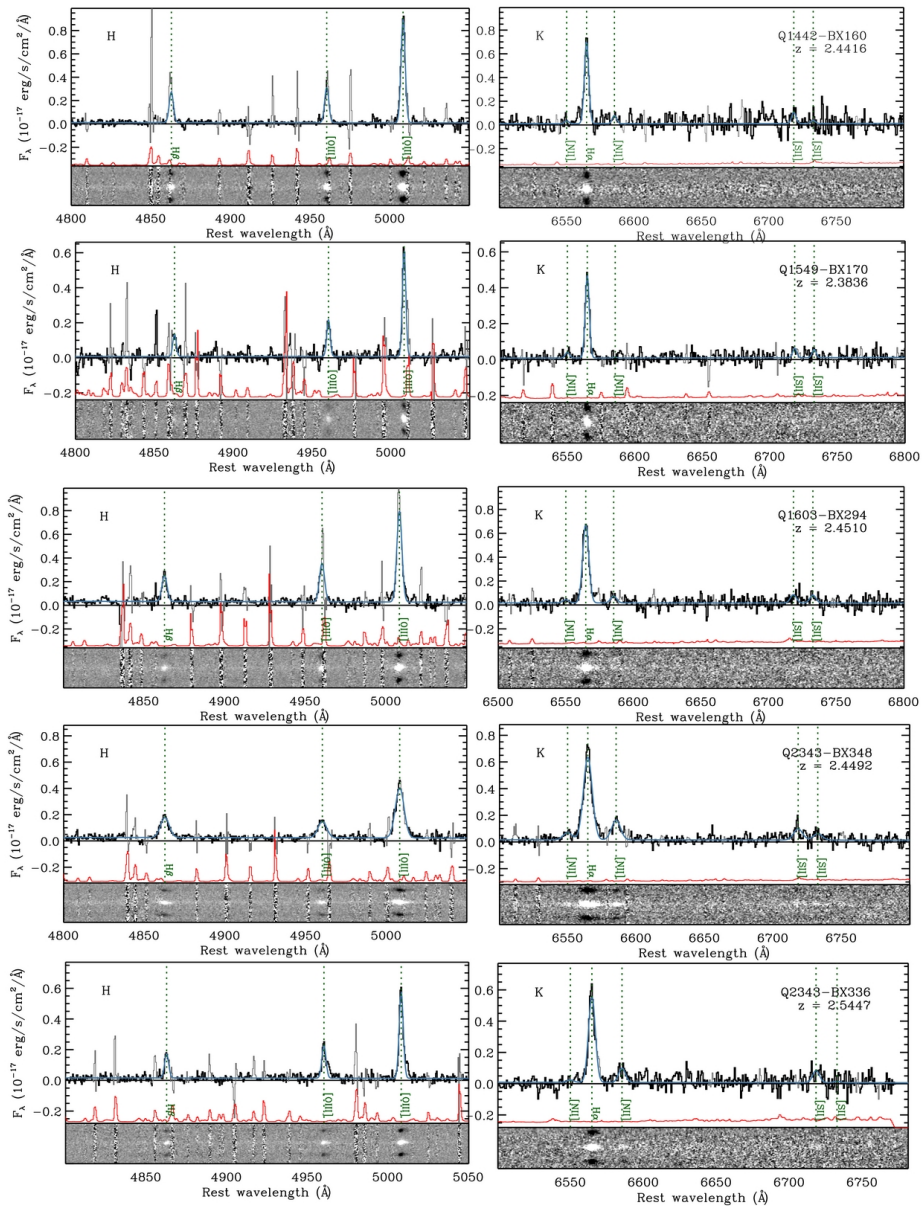
Figure 2. from Strong Nebular Line Ratios in the Spectra of z \sim 2-3 Star Forming Galaxies: First Results from KBSS-MOSFIRE Steidel et al. 2014 ApJ 795 165 doi:10.1088/0004-637X/795/2/165 https://dx.doi.org/10.1088/0004-637X/795/2/165 © 2014. The American Astronomical Society. All rights reserved.
