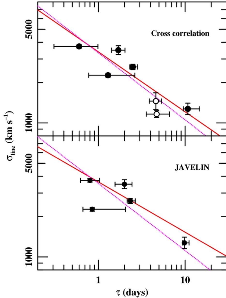
Figure 7. from Reverberation Mapping of the Seyfert 1 Galaxy NGC 7469 Peterson et al. 2014 ApJ 795 149 doi:10.1088/0004-637X/795/2/149 https://dx.doi.org/10.1088/0004-637X/795/2/149 © 2014. The American Astronomical Society. All rights reserved.
