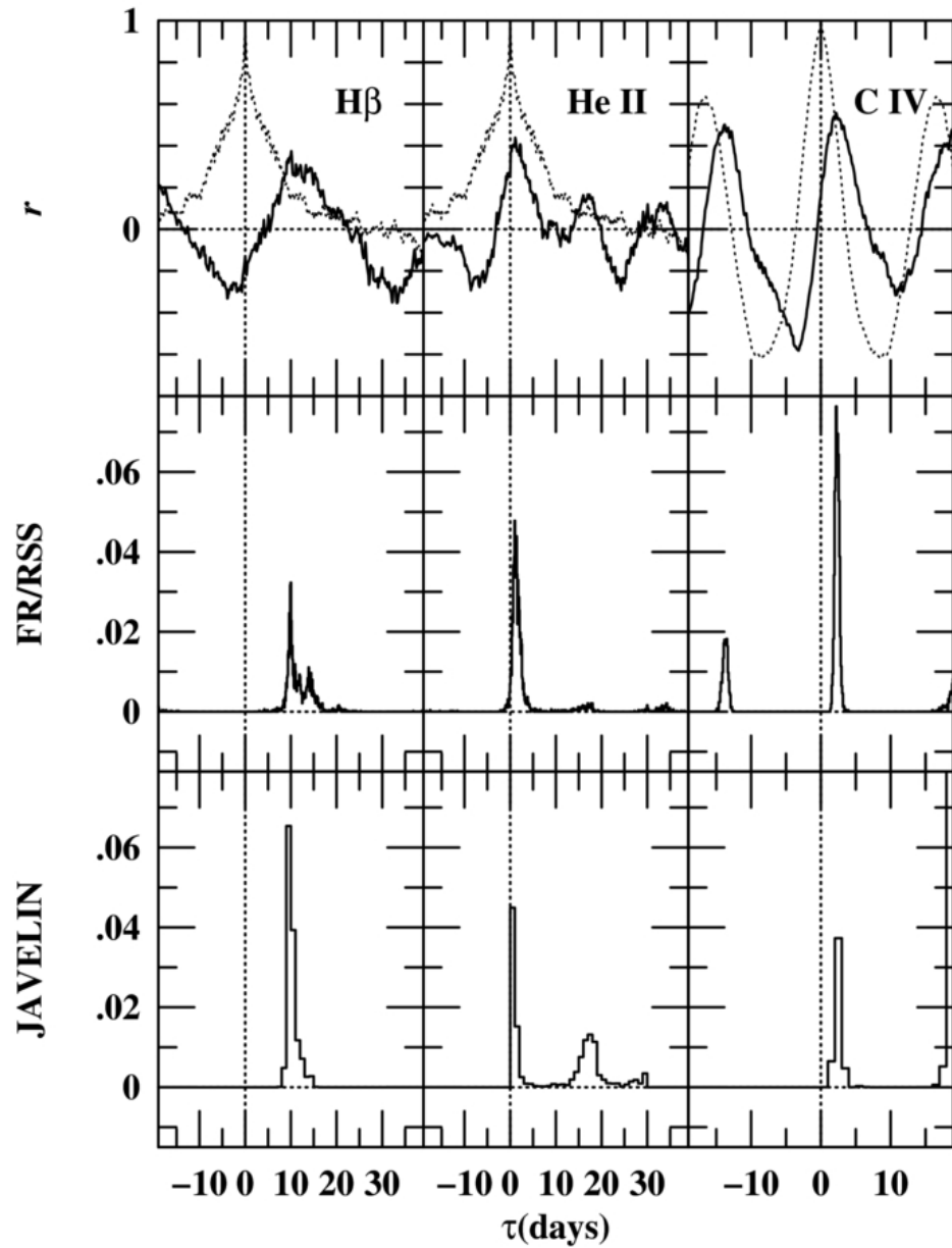
Figure 6. from Reverberation Mapping of the Seyfert 1 Galaxy NGC 7469 Peterson et al. 2014 ApJ 795 149 doi:10.1088/0004-637X/795/2/149 https://dx.doi.org/10.1088/0004-637X/795/2/149 © 2014. The American Astronomical Society. All rights reserved.
