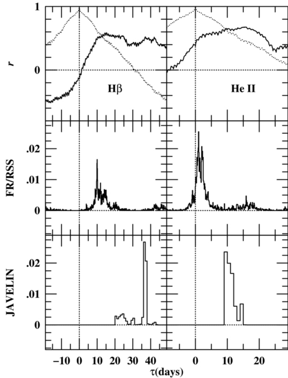
Figure 4. from Reverberation Mapping of the Seyfert 1 Galaxy NGC 7469 Peterson et al. 2014 ApJ 795 149 doi:10.1088/0004-637X/795/2/149 https://dx.doi.org/10.1088/0004-637X/795/2/149 © 2014. The American Astronomical Society. All rights reserved.
