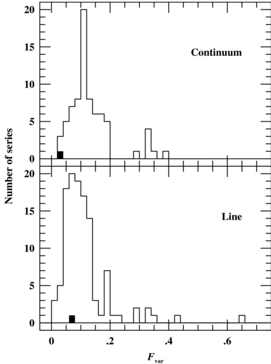
Figure 3. from Reverberation Mapping of the Seyfert 1 Galaxy NGC 7469 Peterson et al. 2014 ApJ 795 149 doi:10.1088/0004-637X/795/2/149 https://dx.doi.org/10.1088/0004-637X/795/2/149 © 2014. The American Astronomical Society. All rights reserved.
