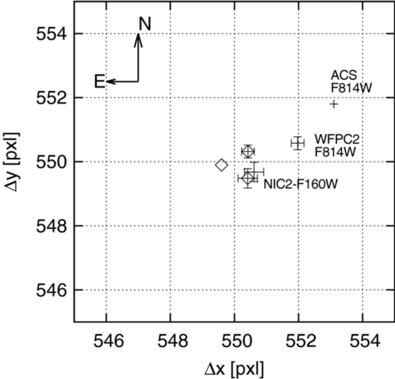
Figure 8. from Recoiling Supermassive Black Holes: A Search in the Nearby Universe Lena et al. 2014 ApJ 795 146 doi:10.1088/0004-637X/795/2/146 https://dx.doi.org/10.1088/0004-637X/795/2/146 © 2014. The American Astronomical Society. All rights reserved.
