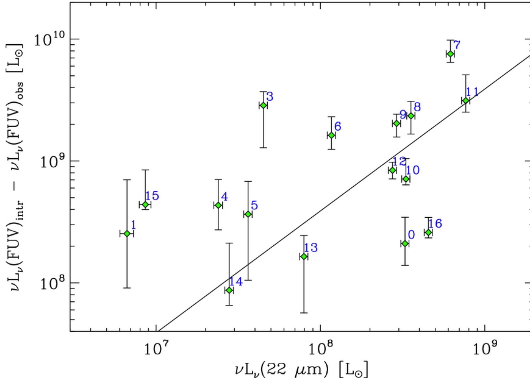
Figure 8. from Star Formation Histories across the Interacting Galaxy NGC 6872, the Largest-known Spiral Eufrasio et al. 2014 ApJ 795 89 doi:10.1088/0004-637X/795/1/89 https://dx.doi.org/10.1088/0004-637X/795/1/89 © 2014. The American Astronomical Society. All rights reserved.
