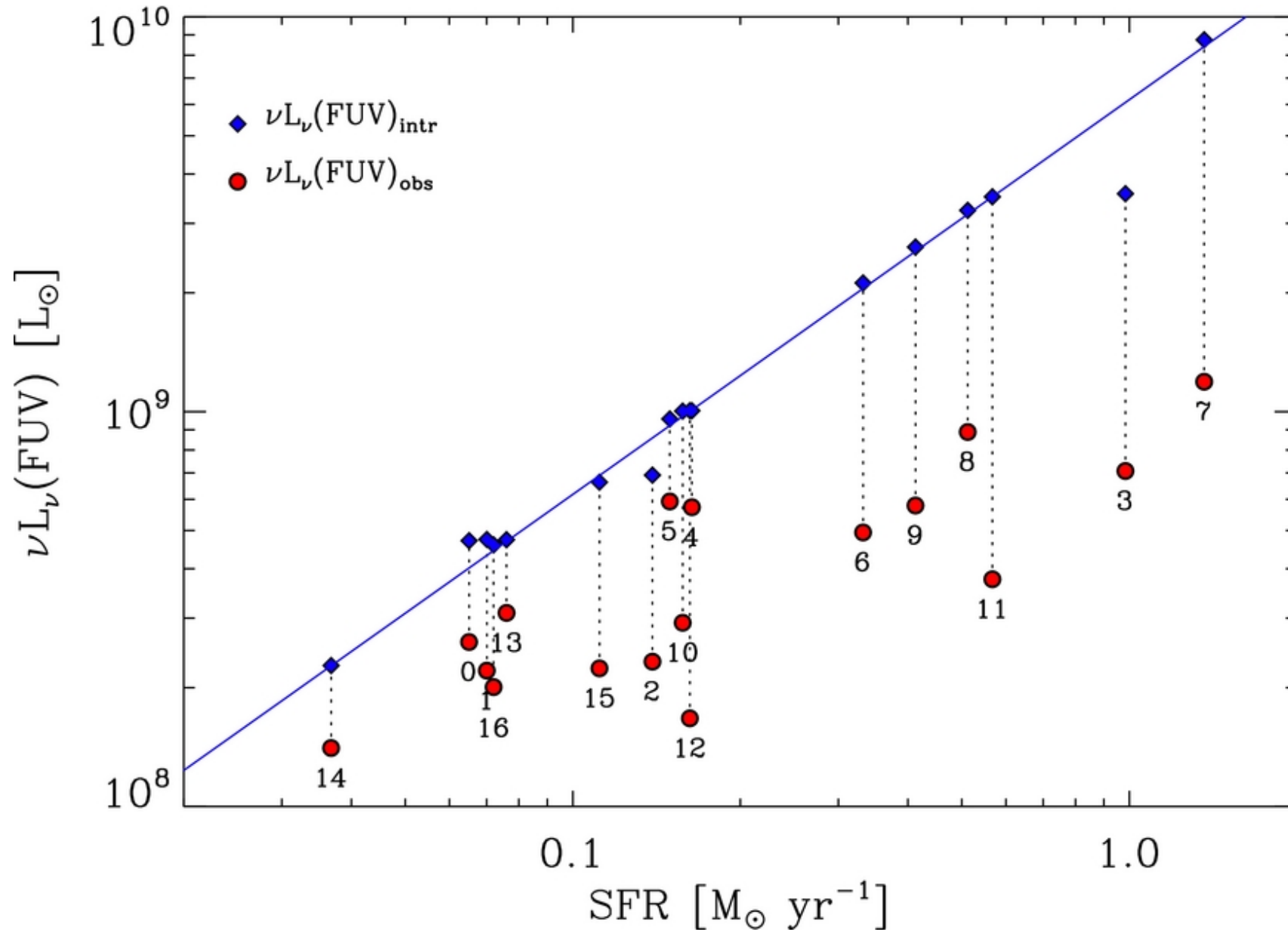
Figure 7. from Star Formation Histories across the Interacting Galaxy NGC 6872, the Largest-known Spiral Eufrasio et al. 2014 ApJ 795 89 doi:10.1088/0004-637X/795/1/89 https://dx.doi.org/10.1088/0004-637X/795/1/89 © 2014. The American Astronomical Society. All rights reserved.
