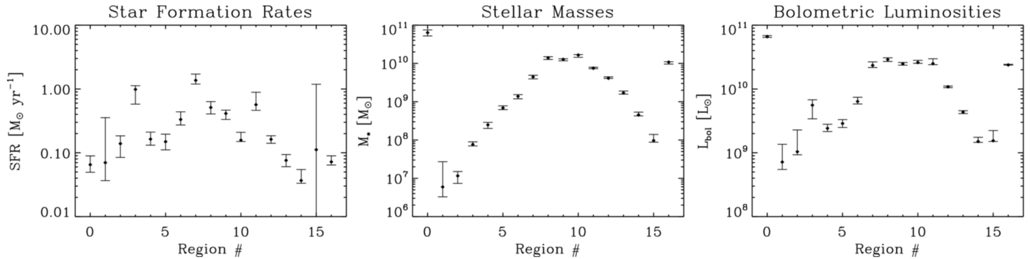
Figure 6. from Star Formation Histories across the Interacting Galaxy NGC 6872, the Largest-known Spiral Eufrasio et al. 2014 ApJ 795 89 doi:10.1088/0004-637X/795/1/89 https://dx.doi.org/10.1088/0004-637X/795/1/89
