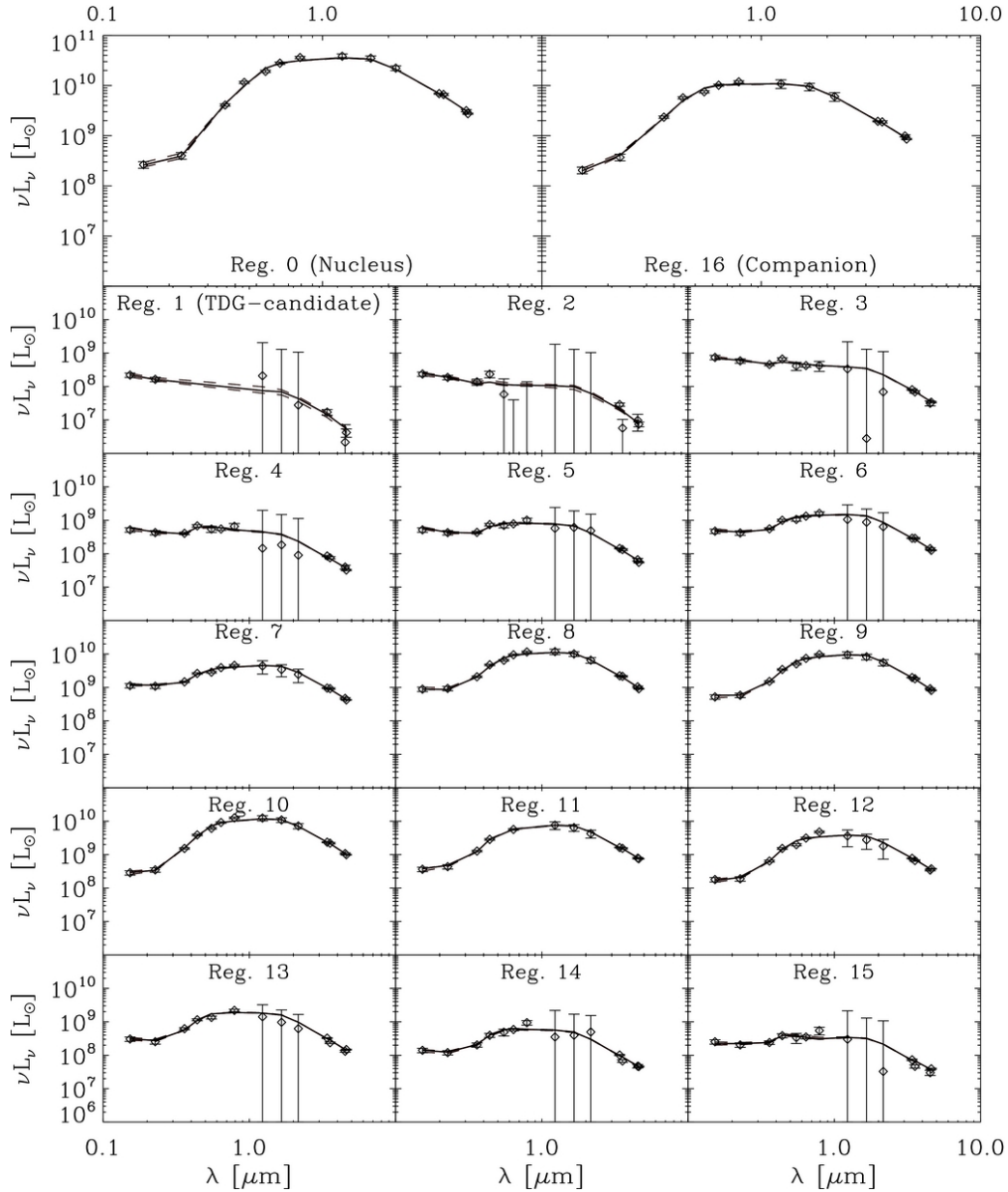
Figure 4. from Star Formation Histories across the Interacting Galaxy NGC 6872, the Largest-known Spiral Eufrasio et al. 2014 ApJ 795 89 doi:10.1088/0004-637X/795/1/89 https://dx.doi.org/10.1088/0004-637X/795/1/89
