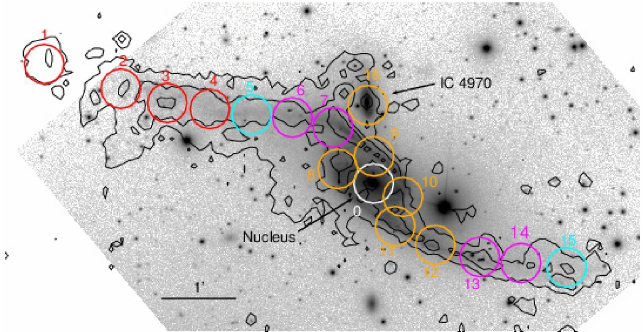
Figure 2. from Star Formation Histories across the Interacting Galaxy NGC 6872, the Largest-known Spiral Eufrasio et al. 2014 ApJ 795 89 doi:10.1088/0004-637X/795/1/89 https://dx.doi.org/10.1088/0004-637X/795/1/89 © 2014. The American Astronomical Society. All rights reserved.
