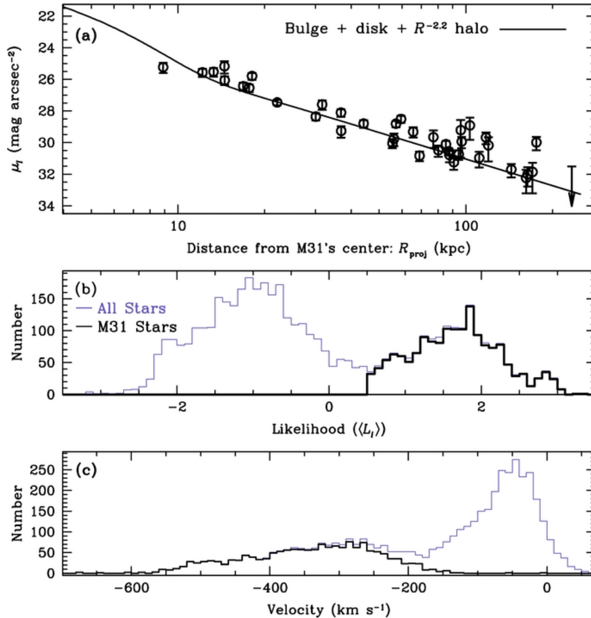
Figure 2. from Global Properties of M31's Stellar Halo from the SPLASH Survey. II. Metallicity Profile Gilbert et al. 2014 ApJ 796 76 doi:10.1088/0004-637X/796/2/76 https://dx.doi.org/10.1088/0004-637X/796/2/76 © 2014. The American Astronomical Society. All rights reserved.
