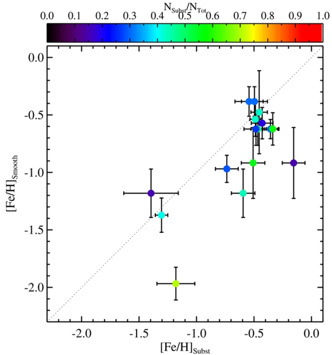
Figure 14. from Global Properties of M31's Stellar Halo from the SPLASH Survey. II. Metallicity Profile Gilbert et al. 2014 ApJ 796 76 doi:10.1088/0004-637X/796/2/76 https://dx.doi.org/10.1088/0004-637X/796/2/76 © 2014. The American Astronomical Society. All rights reserved.
