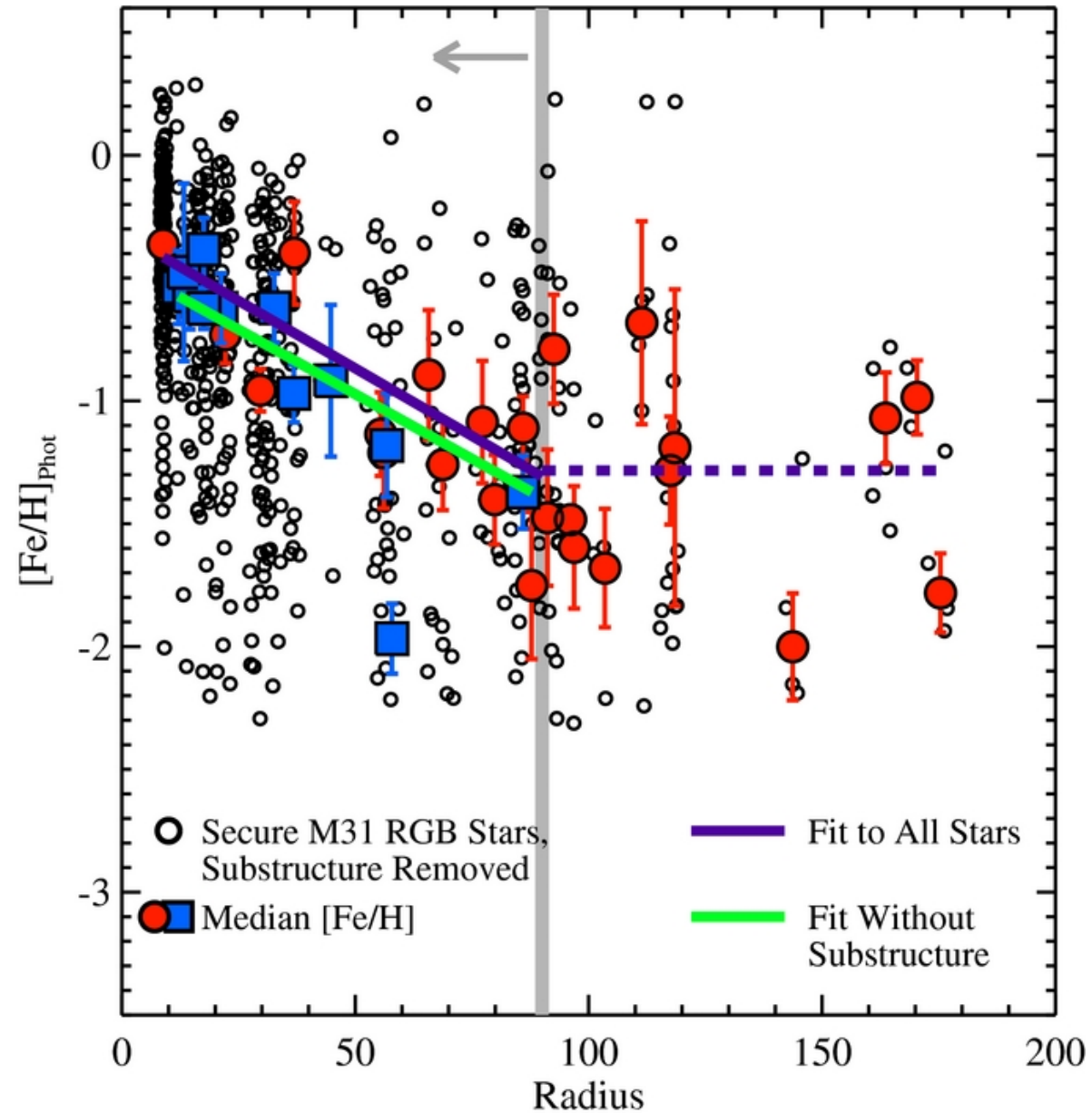
Figure 10. from Global Properties of M31's Stellar Halo from the SPLASH Survey. II. Metallicity Profile Gilbert et al. 2014 ApJ 796 76 doi:10.1088/0004-637X/796/2/76 https://dx.doi.org/10.1088/0004-637X/796/2/76 © 2014. The American Astronomical Society. All rights reserved.
