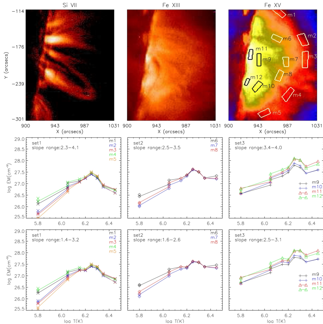
Figure 5. from Emission Measure Distribution for Diffuse Regions in Solar Active Regions Subramanian et al. 2014 ApJ 795 76 doi:10.1088/0004-637X/795/1/76 https://dx.doi.org/10.1088/0004-637X/795/1/76 © 2014. The American Astronomical Society. All rights reserved.
