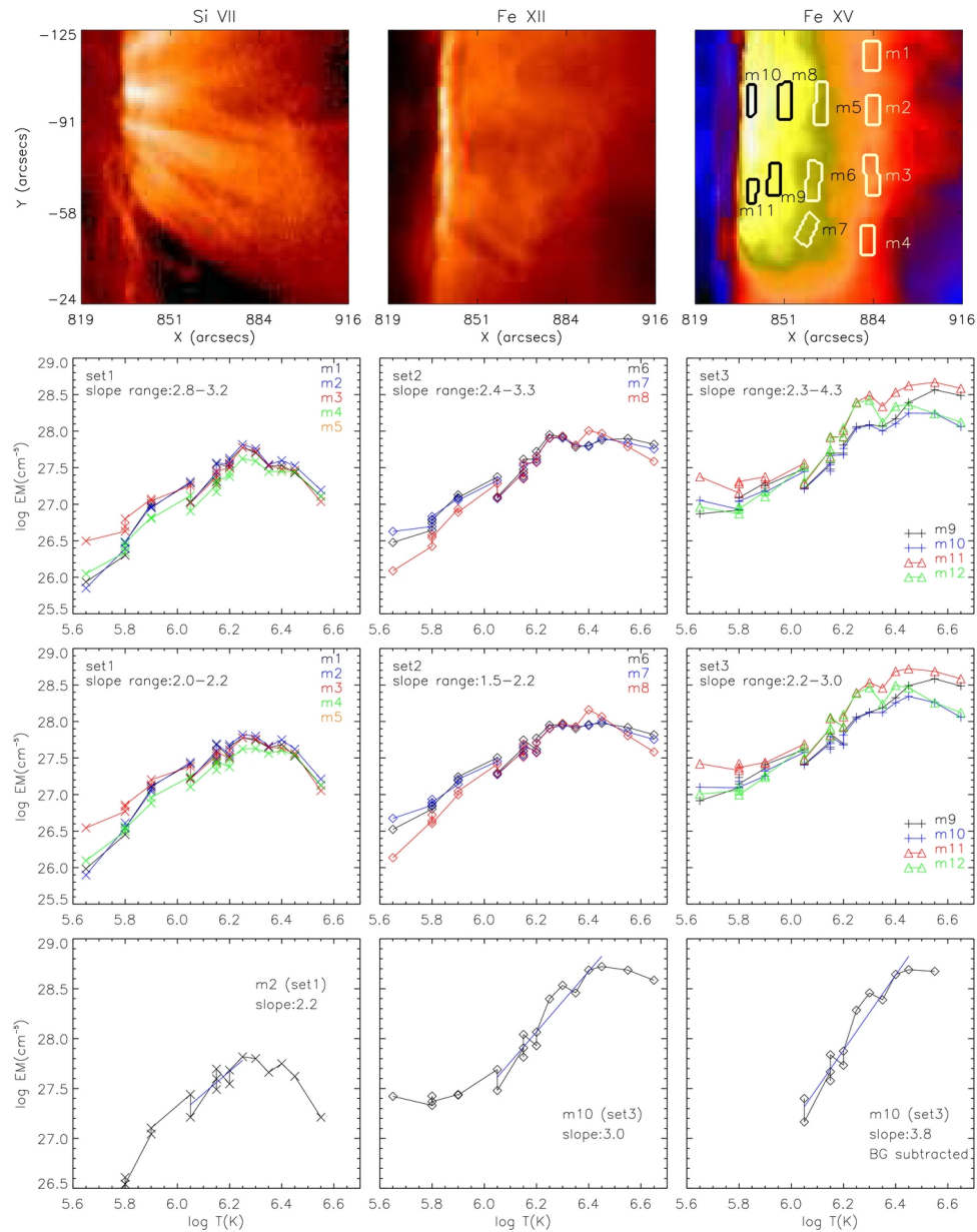
Figure 4. from Emission Measure Distribution for Diffuse Regions in Solar Active Regions Subramanian et al. 2014 ApJ 795 76 doi:10.1088/0004-637X/795/1/76 https://dx.doi.org/10.1088/0004-637X/795/1/76
