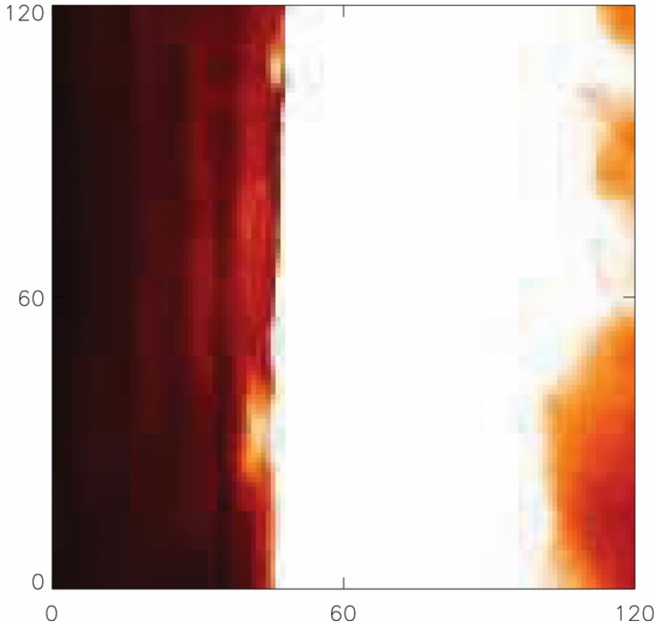
Figure 2. from Emission Measure Distribution for Diffuse Regions in Solar Active Regions Subramanian et al. 2014 ApJ 795 76 doi:10.1088/0004-637X/795/1/76 https://dx.doi.org/10.1088/0004-637X/795/1/76 © 2014. The American Astronomical Society. All rights reserved.
