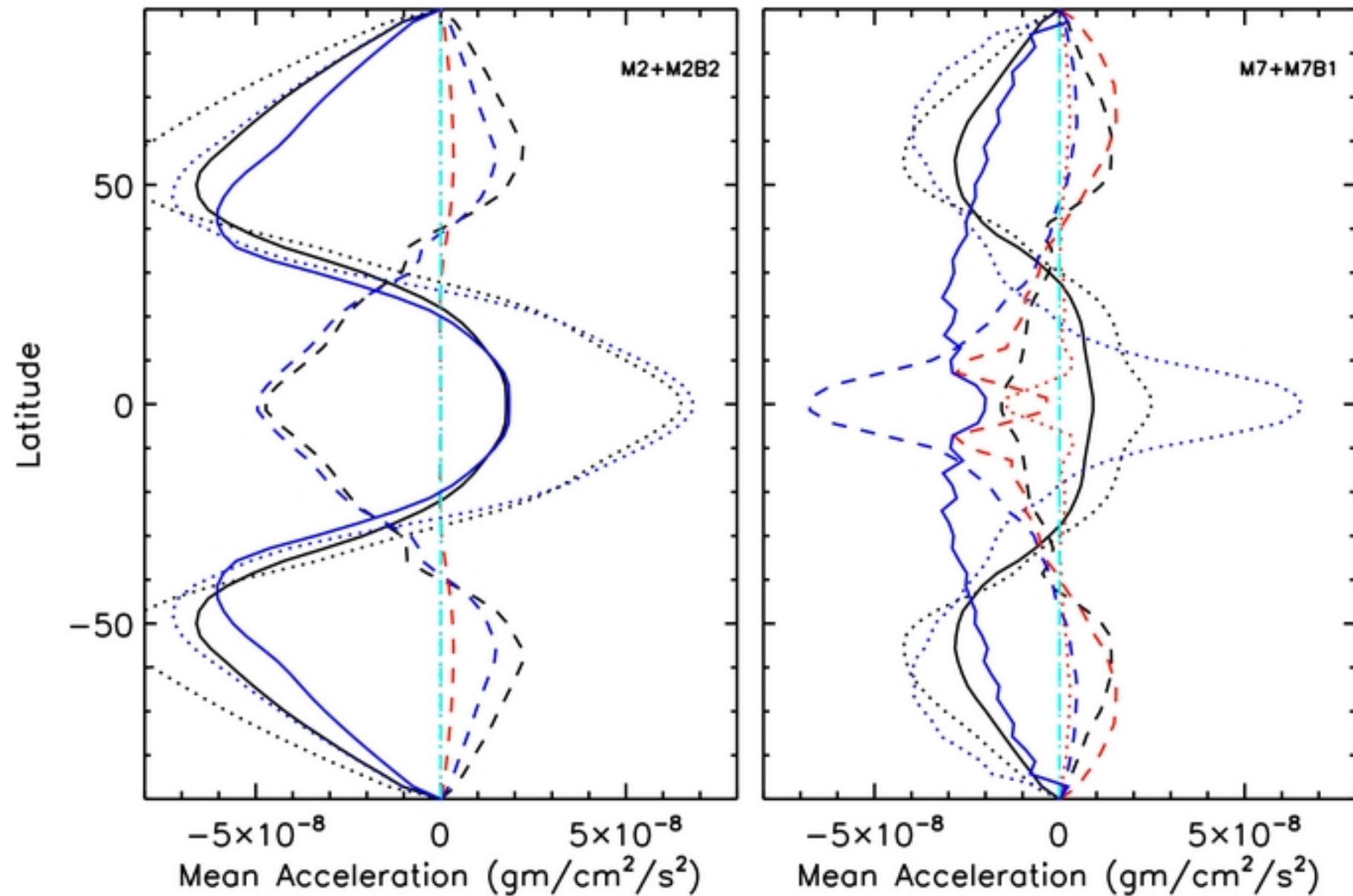
Figure 9. from Magnetic Effects in Hot Jupiter Atmospheres Rogers & Komacek 2014 ApJ 794 132 doi:10.1088/0004-637X/794/2/132 https://dx.doi.org/10.1088/0004-637X/794/2/132 © 2014. The American Astronomical Society. All rights reserved.
