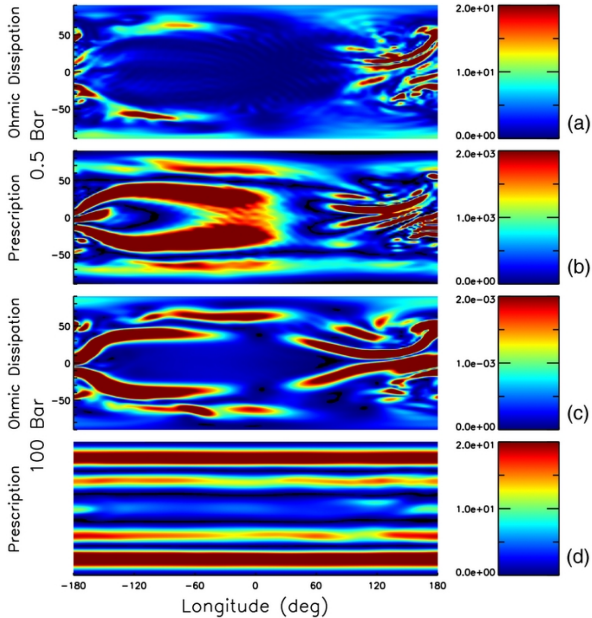
Figure 8. from Magnetic Effects in Hot Jupiter Atmospheres Rogers & Komacek 2014 ApJ 794 132 doi:10.1088/0004-637X/794/2/132 https://dx.doi.org/10.1088/0004-637X/794/2/132 © 2014. The American Astronomical Society. All rights reserved.
