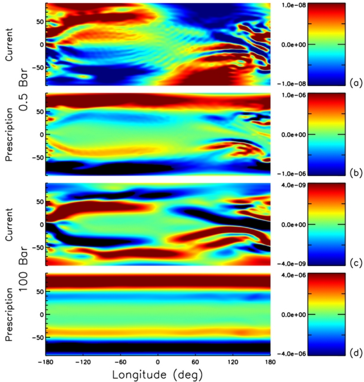
Figure 7. from Magnetic Effects in Hot Jupiter Atmospheres Rogers & Komacek 2014 ApJ 794 132 doi:10.1088/0004-637X/794/2/132 https://dx.doi.org/10.1088/0004-637X/794/2/132 © 2014. The American Astronomical Society. All rights reserved.
