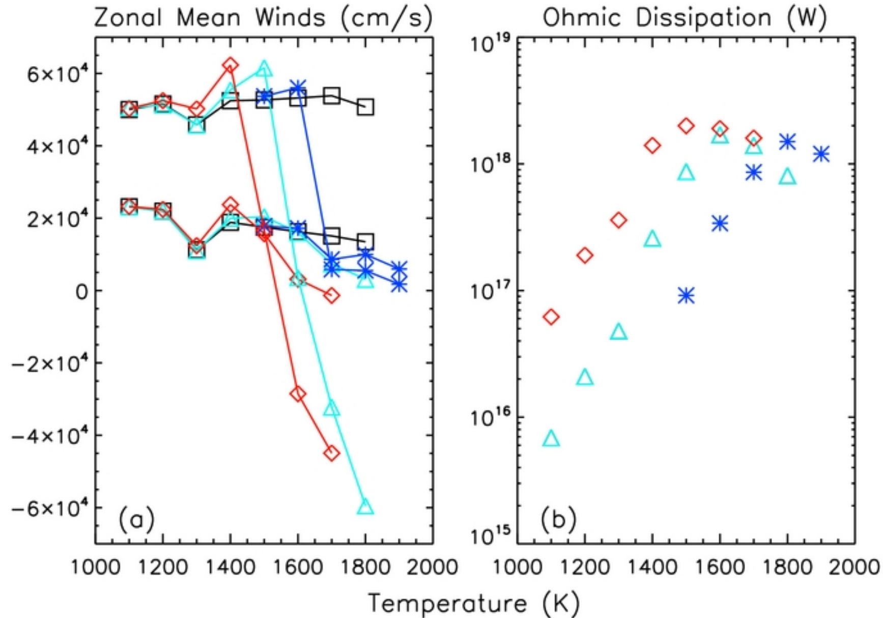
Figure 6. from Magnetic Effects in Hot Jupiter Atmospheres Rogers & Komacek 2014 ApJ 794 132 doi:10.1088/0004-637X/794/2/132 https://dx.doi.org/10.1088/0004-637X/794/2/132 © 2014. The American Astronomical Society. All rights reserved.
