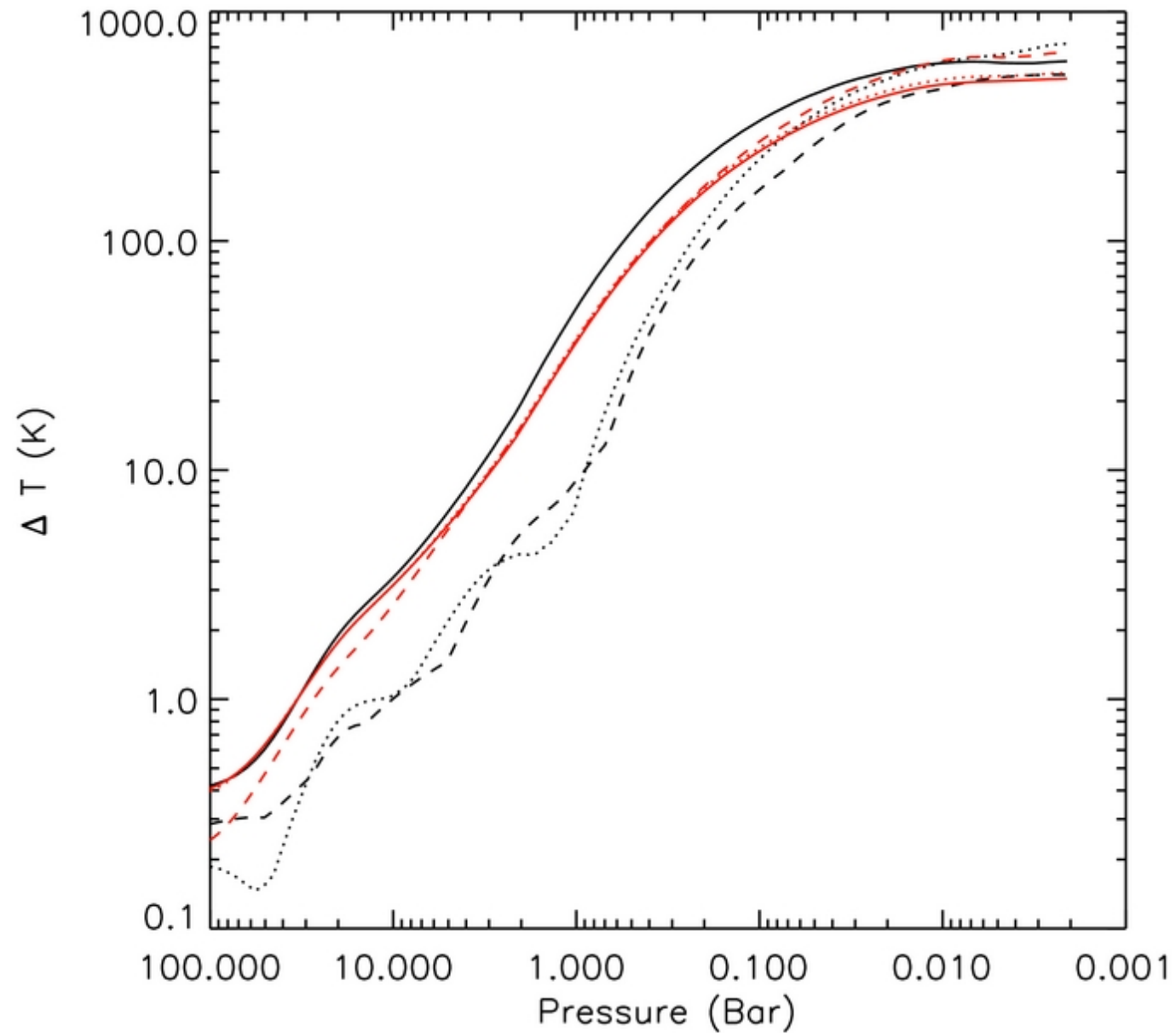
Figure 5. from Magnetic Effects in Hot Jupiter Atmospheres Rogers & Komacek 2014 ApJ 794 132 doi:10.1088/0004-637X/794/2/132 https://dx.doi.org/10.1088/0004-637X/794/2/132 © 2014. The American Astronomical Society. All rights reserved.
