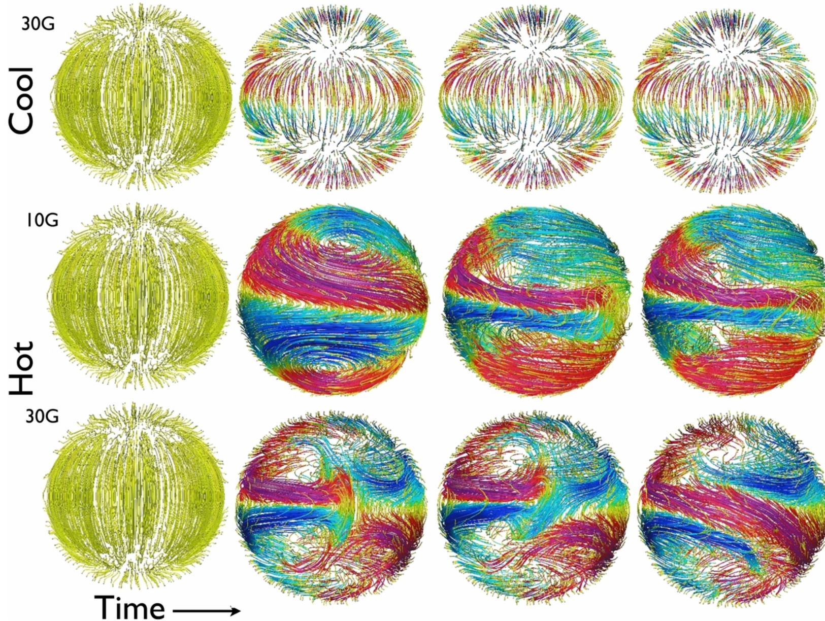
Figure 3. from Magnetic Effects in Hot Jupiter Atmospheres Rogers & Komacek 2014 ApJ 794 132 doi:10.1088/0004-637X/794/2/132 https://dx.doi.org/10.1088/0004-637X/794/2/132 © 2014. The American Astronomical Society. All rights reserved.
