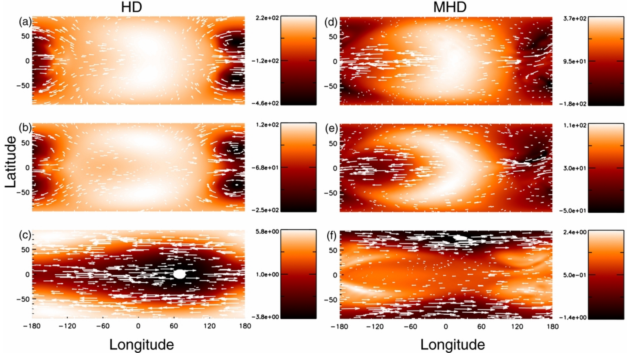
Figure 2. from Magnetic Effects in Hot Jupiter Atmospheres Rogers & Komacek 2014 ApJ 794 132 doi:10.1088/0004-637X/794/2/132 https://dx.doi.org/10.1088/0004-637X/794/2/132 © 2014. The American Astronomical Society. All rights reserved.
