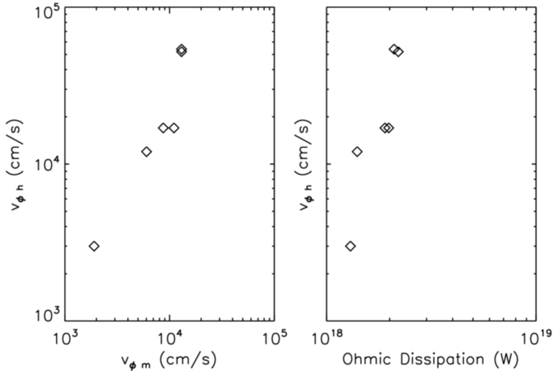
Figure 13. from Magnetic Effects in Hot Jupiter Atmospheres Rogers & Komacek 2014 ApJ 794 132 doi:10.1088/0004-637X/794/2/132 https://dx.doi.org/10.1088/0004-637X/794/2/132 © 2014. The American Astronomical Society. All rights reserved.
