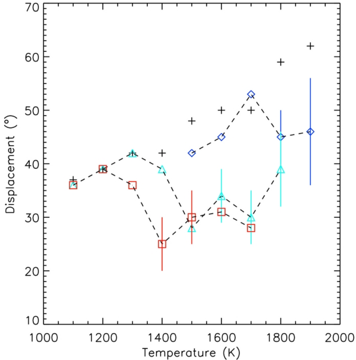
Figure 12. from Magnetic Effects in Hot Jupiter Atmospheres Rogers & Komacek 2014 ApJ 794 132 doi:10.1088/0004-637X/794/2/132 https://dx.doi.org/10.1088/0004-637X/794/2/132 © 2014. The American Astronomical Society. All rights reserved.
