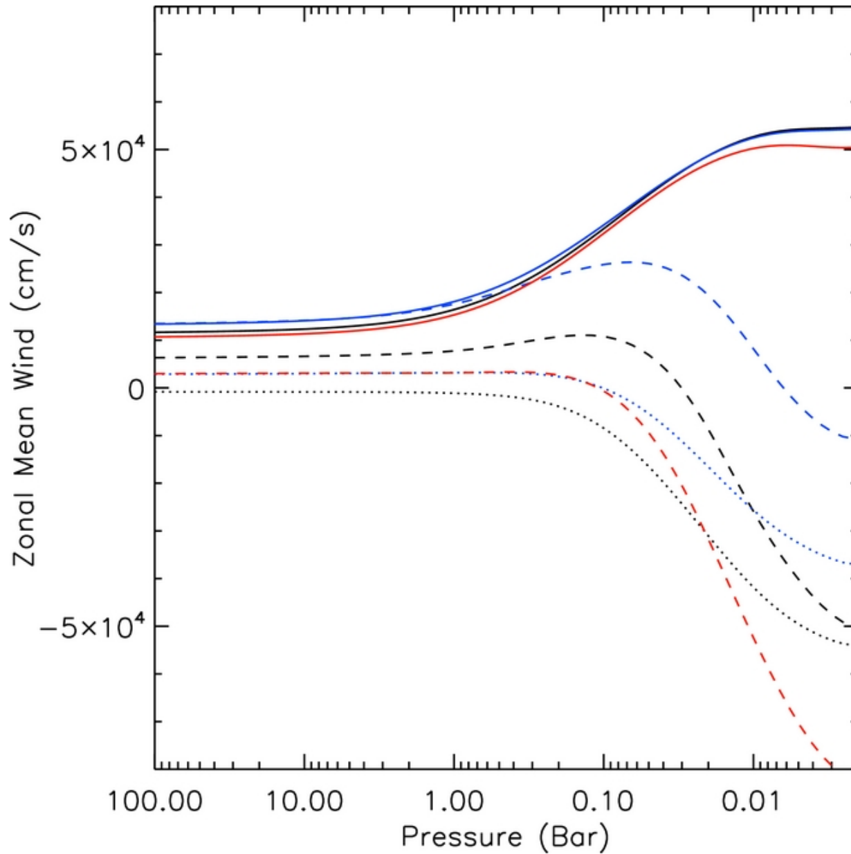
Figure 11. from Magnetic Effects in Hot Jupiter Atmospheres Rogers & Komacek 2014 ApJ 794 132 doi:10.1088/0004-637X/794/2/132 https://dx.doi.org/10.1088/0004-637X/794/2/132 © 2014. The American Astronomical Society. All rights reserved.
