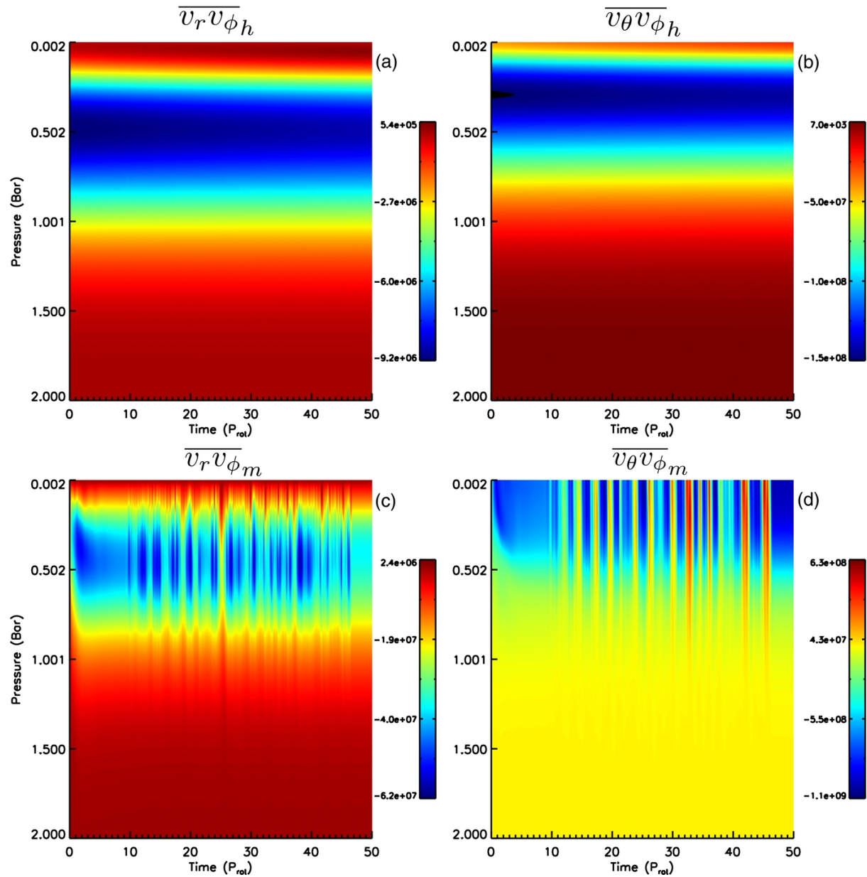
Figure 10. from Magnetic Effects in Hot Jupiter Atmospheres Rogers & Komacek 2014 ApJ 794 132 doi:10.1088/0004-637X/794/2/132 https://dx.doi.org/10.1088/0004-637X/794/2/132 © 2014. The American Astronomical Society. All rights reserved.
