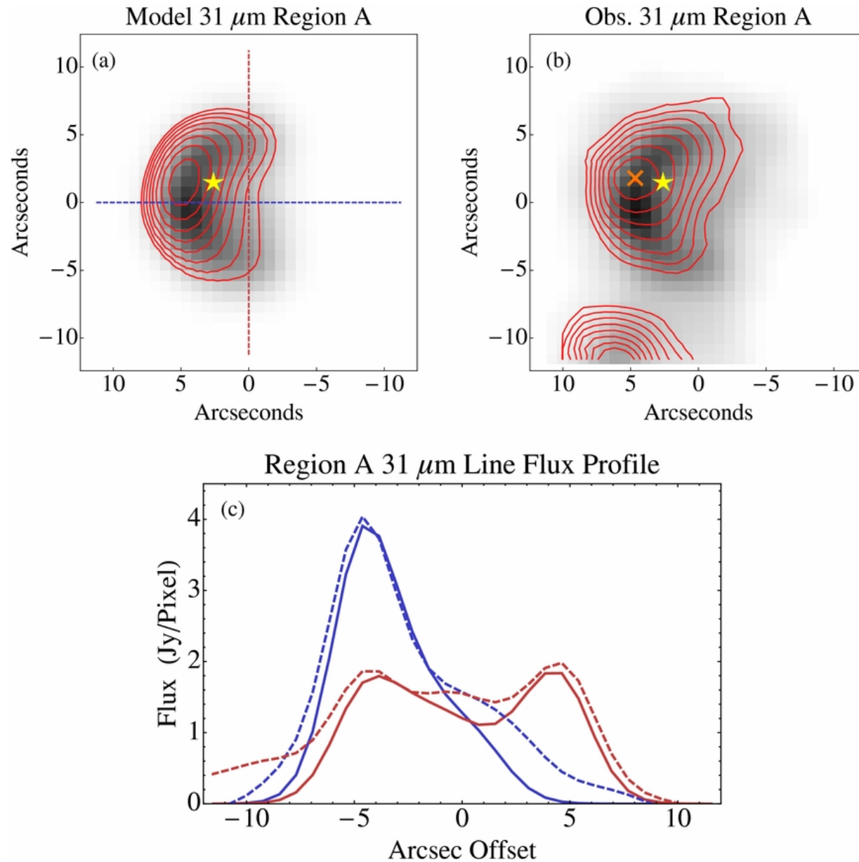
Figure 7. from Dusty Cradles in a Turbulent Nursery: The Sgr A East H II Region Complex at the Galactic Center Lau et al. 2014 ApJ 794 108 doi:10.1088/0004-637X/794/2/108 https://dx.doi.org/10.1088/0004-637X/794/2/108 © 2014. The American Astronomical Society. All rights reserved.
