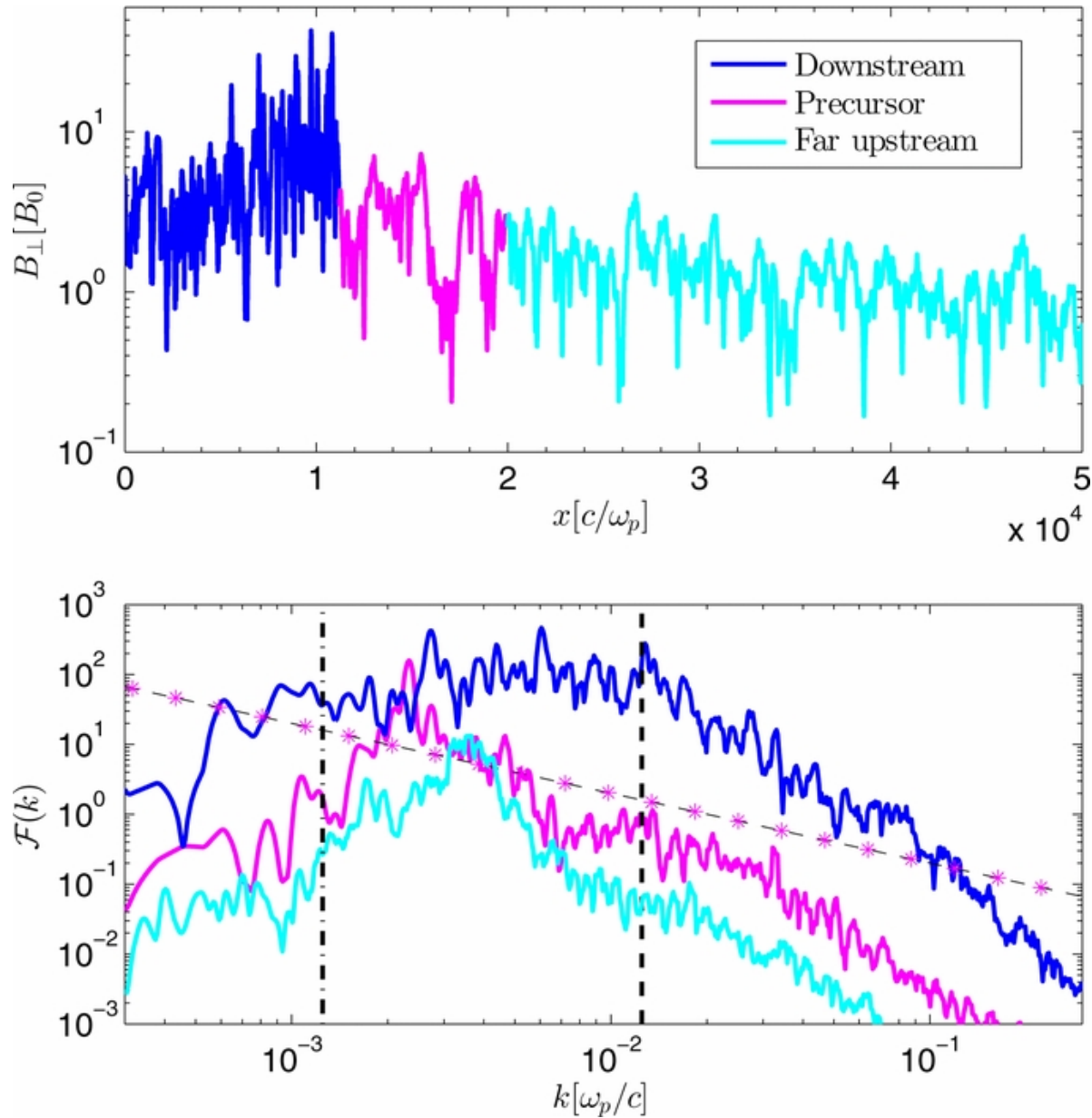
Figure 7. from Simulations of Ion Acceleration at Non-relativistic Shocks. II. Magnetic Field Amplification Caprioli & Spitkovsky 2014 ApJ 794 46 doi:10.1088/0004-637X/794/1/46 https://dx.doi.org/10.1088/0004-637X/794/1/46 © 2014. The American Astronomical Society. All rights reserved.
