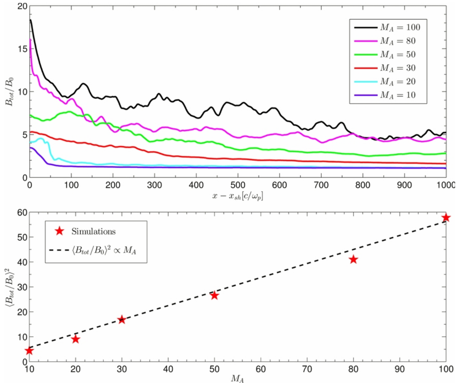
Figure 5. from Simulations of Ion Acceleration at Non-relativistic Shocks. II. Magnetic Field Amplification Caprioli & Spitkovsky 2014 ApJ 794 46 doi:10.1088/0004-637X/794/1/46 https://dx.doi.org/10.1088/0004-637X/794/1/46 © 2014. The American Astronomical Society. All rights reserved.
