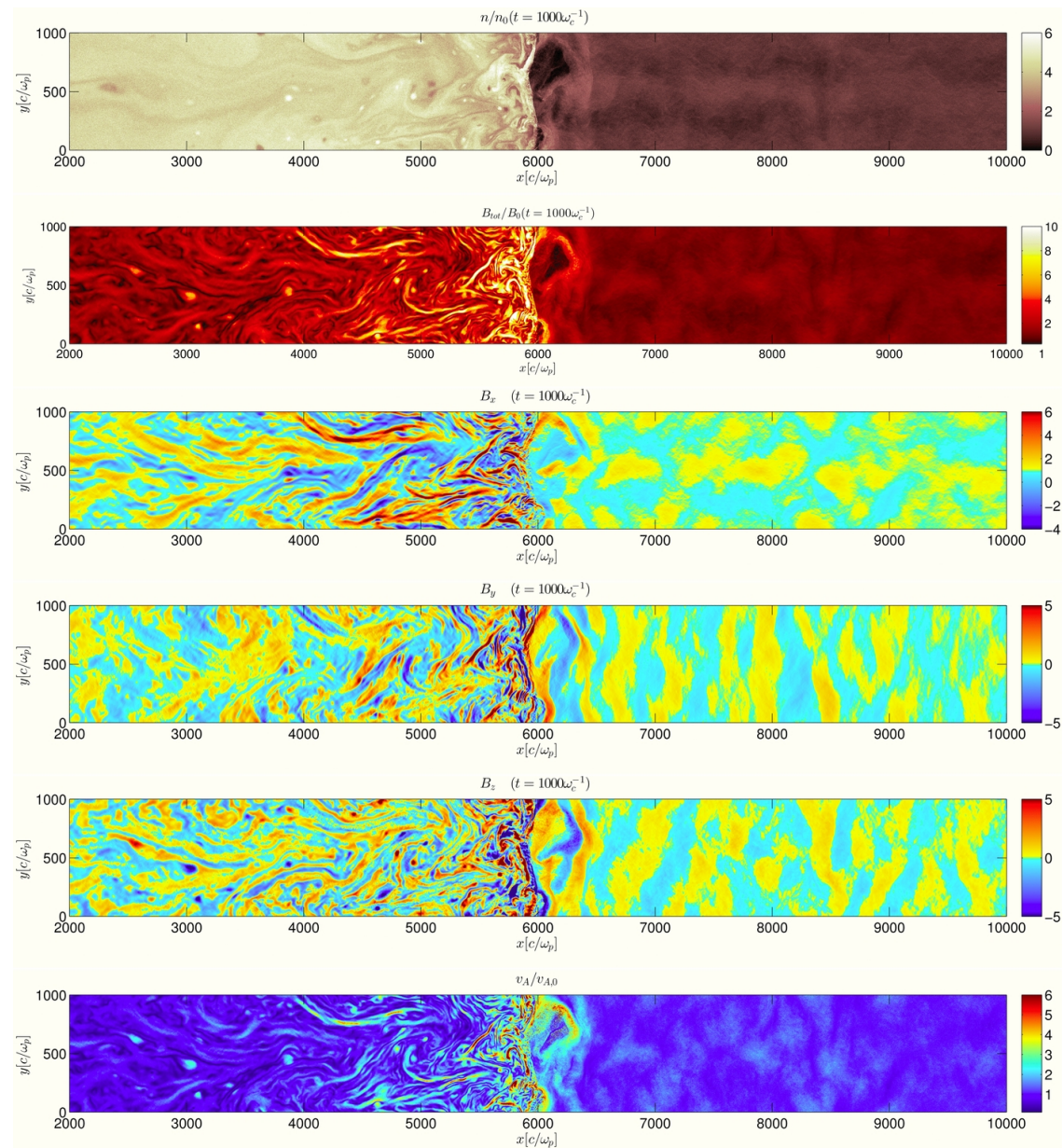
Figure 1. from Simulations of Ion Acceleration at Non-relativistic Shocks. II. Magnetic Field Amplification Caprioli & Spitkovsky 2014 ApJ 794 46 doi:10.1088/0004-637X/794/1/46 https://dx.doi.org/10.1088/0004-637X/794/1/46 © 2014. The American Astronomical Society. All rights reserved.
