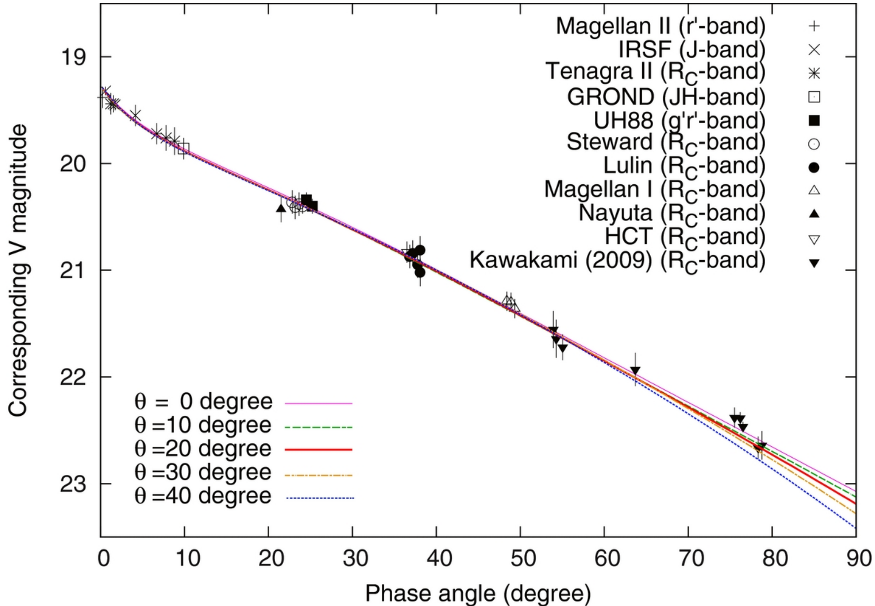
Figure 4. from Optical Properties of (162173) 1999 JU3: In Preparation for the JAXA Hayabusa 2 Sample Return Mission Ishiguro et al. 2014 ApJ 792 74 doi:10.1088/0004-637X/792/1/74 https://dx.doi.org/10.1088/0004-637X/792/1/74 © 2014. The American Astronomical Society. All rights reserved.
