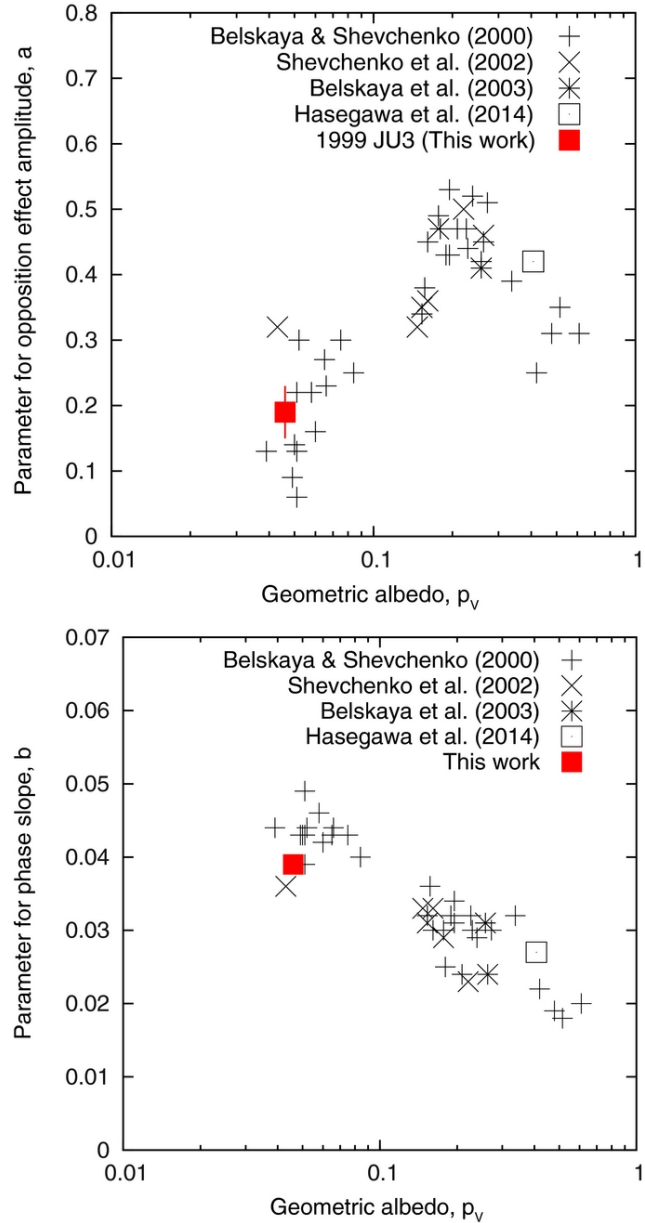
Figure 3. from Optical Properties of (162173) 1999 JU3: In Preparation for the JAXA Hayabusa 2 Sample Return Mission Ishiguro et al. 2014 ApJ 792 74 doi:10.1088/0004-637X/792/1/74 https://dx.doi.org/10.1088/0004-637X/792/1/74
