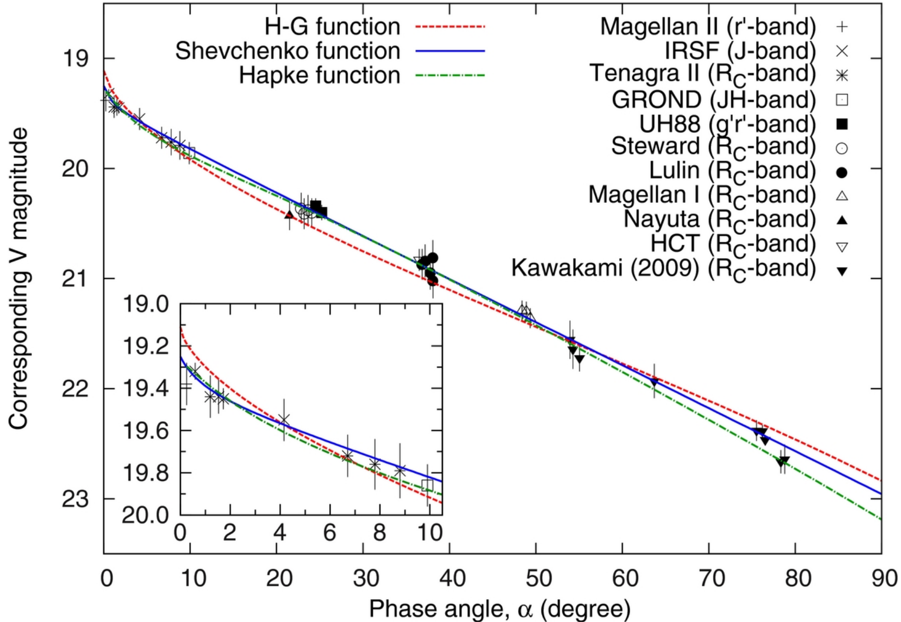
Figure 2. from Optical Properties of (162173) 1999 JU3: In Preparation for the JAXA Hayabusa 2 Sample Return Mission Ishiguro et al. 2014 ApJ 792 74 doi:10.1088/0004-637X/792/1/74 https://dx.doi.org/10.1088/0004-637X/792/1/74 © 2014. The American Astronomical Society. All rights reserved.
