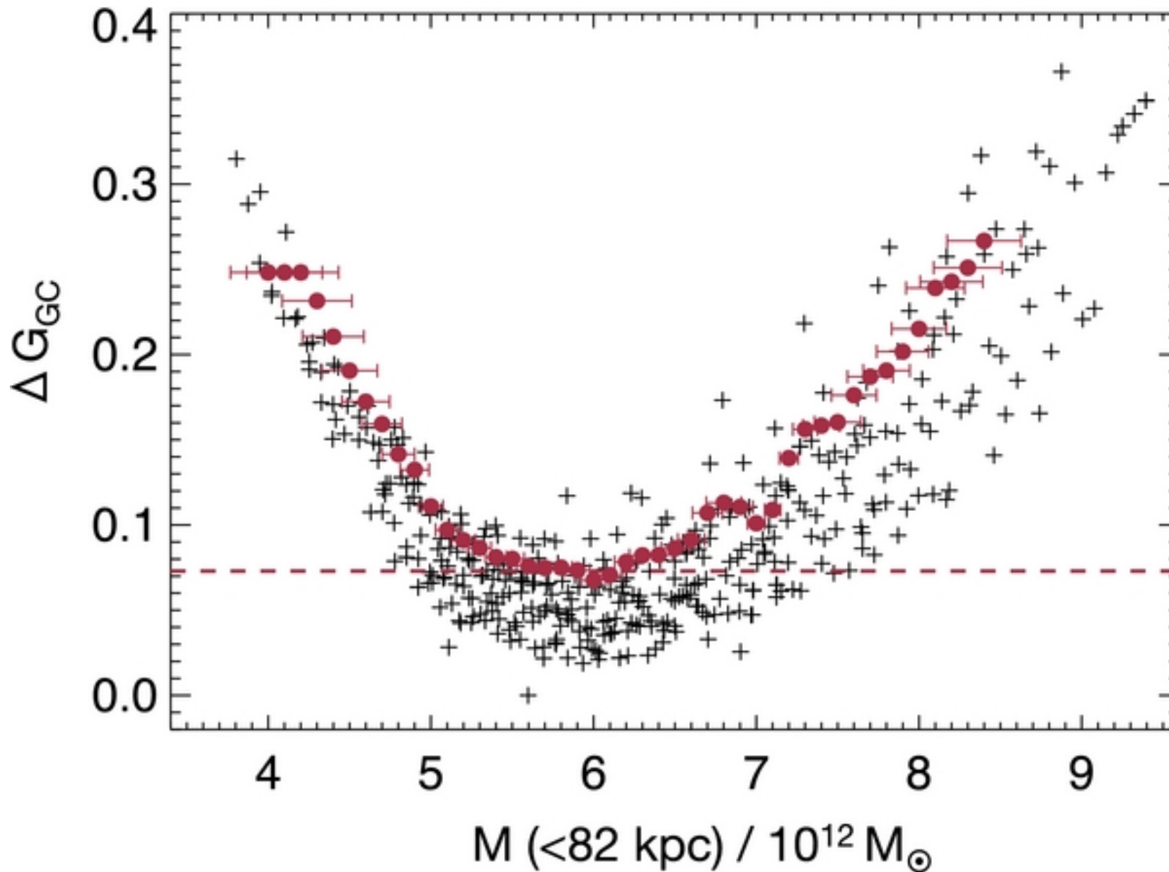
Figure 8. from The Next Generation Virgo Cluster Survey. V. Modeling the Dynamics of M87 with the Made-to-measure Method Zhu et al. 2014 ApJ 792 59 doi:10.1088/0004-637X/792/1/59 https://dx.doi.org/10.1088/0004-637X/792/1/59 © 2014. The American Astronomical Society. All rights reserved.
