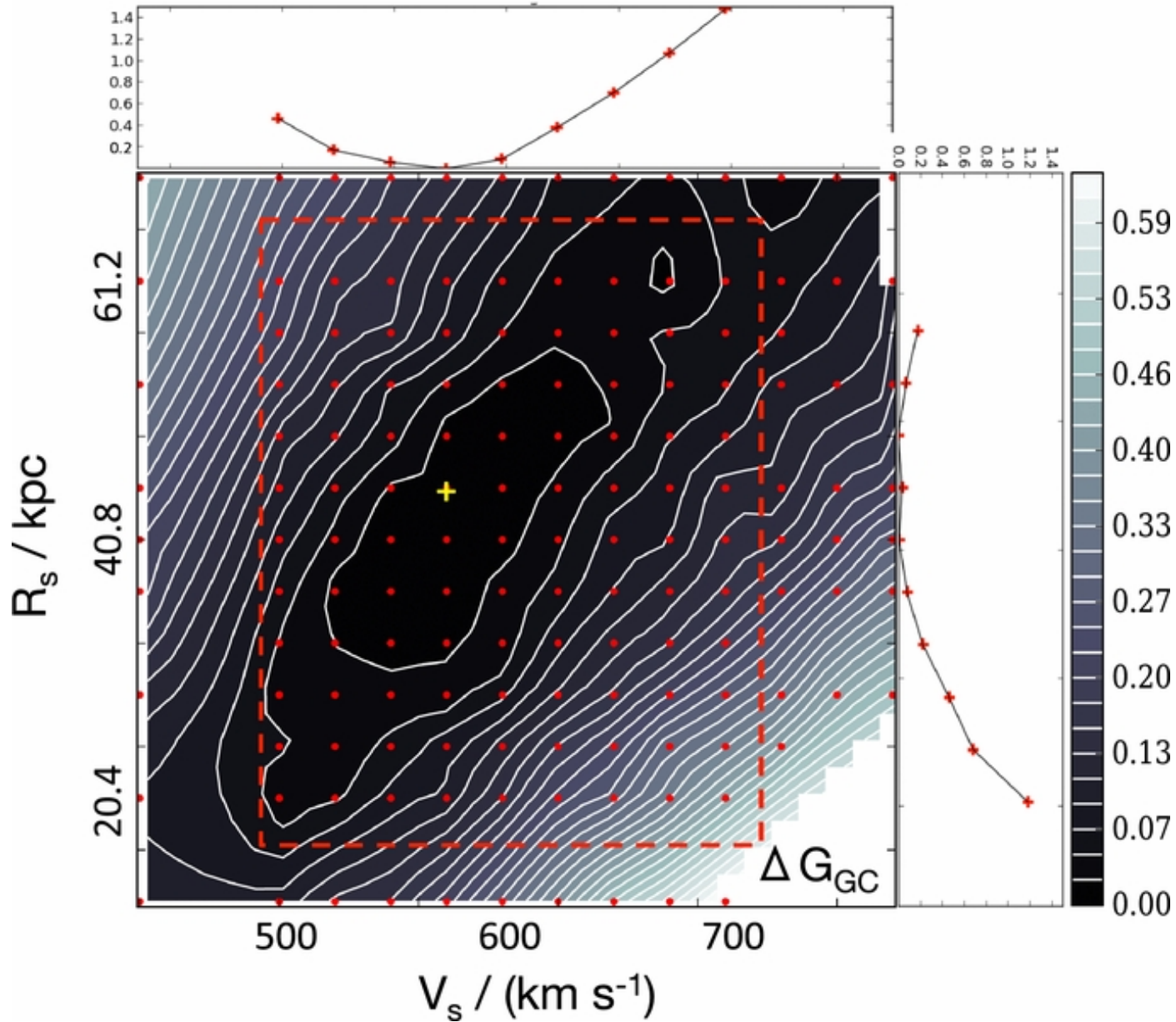
Figure 6. from The Next Generation Virgo Cluster Survey. V. Modeling the Dynamics of M87 with the Made-to-measure Method Zhu et al. 2014 ApJ 792 59 doi:10.1088/0004-637X/792/1/59 https://dx.doi.org/10.1088/0004-637X/792/1/59 © 2014. The American Astronomical Society. All rights reserved.
