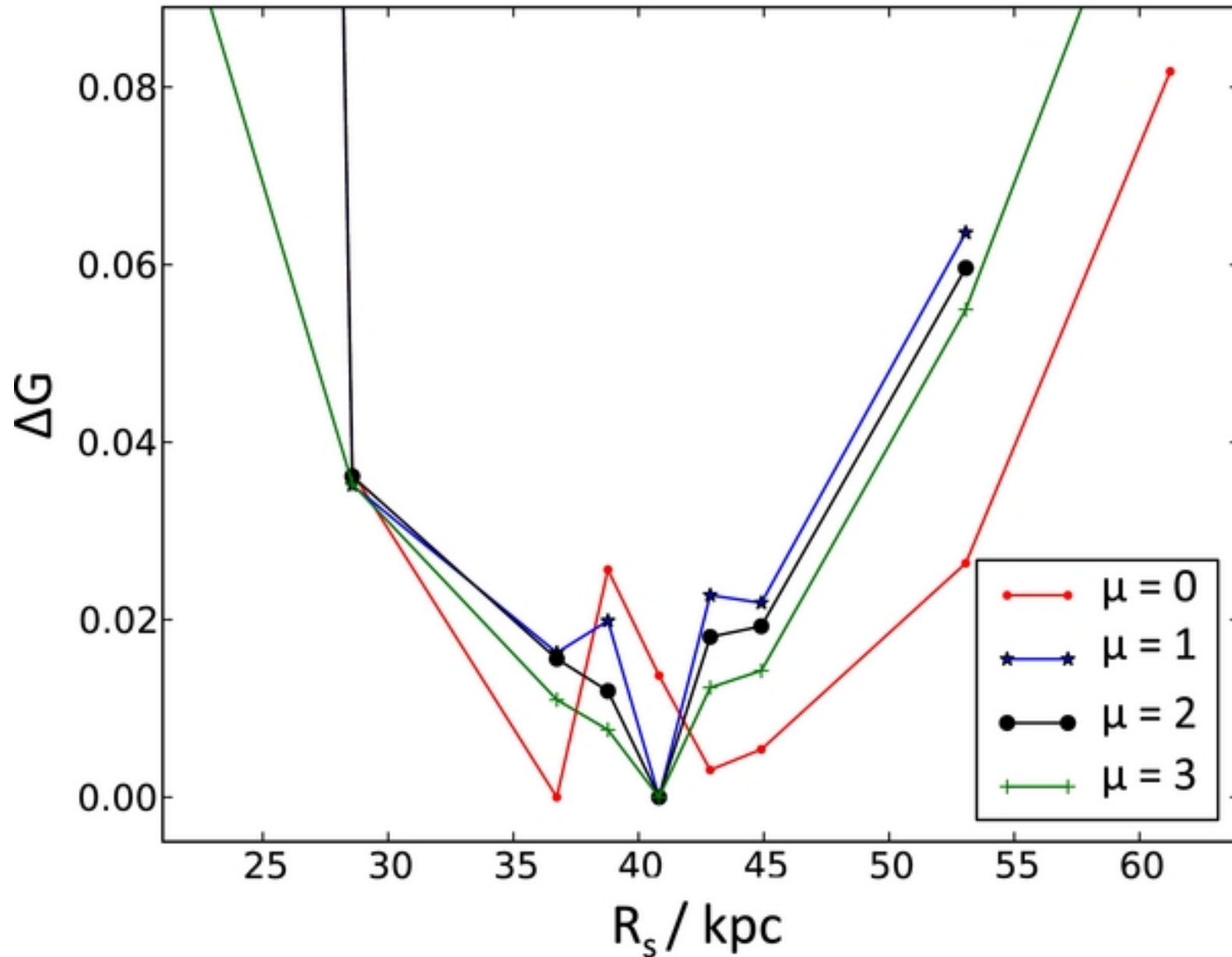
Figure 5. from The Next Generation Virgo Cluster Survey. V. Modeling the Dynamics of M87 with the Made-to-measure Method Zhu et al. 2014 ApJ 792 59 doi:10.1088/0004-637X/792/1/59 https://dx.doi.org/10.1088/0004-637X/792/1/59 © 2014. The American Astronomical Society. All rights reserved.
