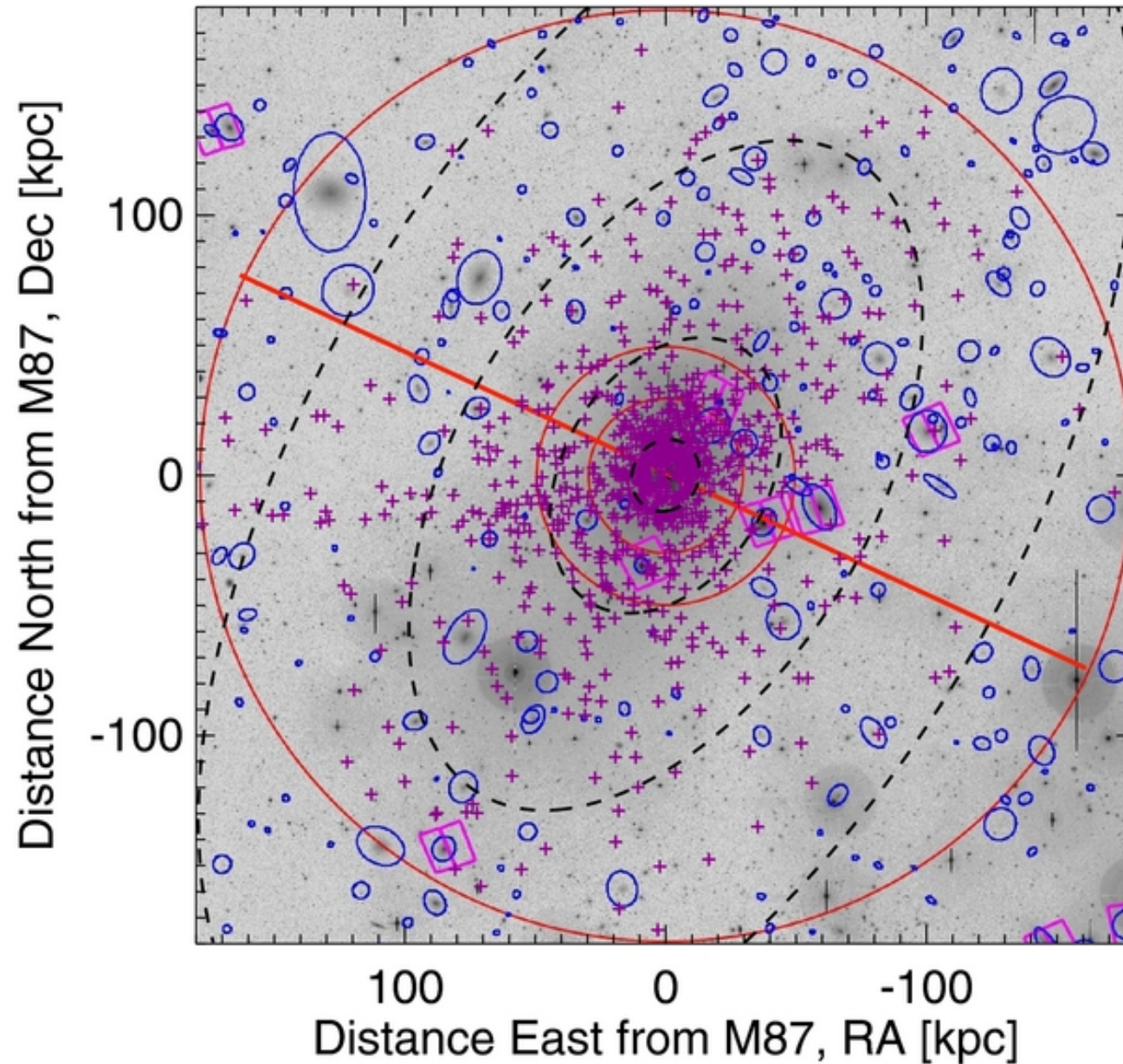
Figure 4. from The Next Generation Virgo Cluster Survey. V. Modeling the Dynamics of M87 with the Made-to-measure Method Zhu et al. 2014 ApJ 792 59 doi:10.1088/0004-637X/792/1/59 https://dx.doi.org/10.1088/0004-637X/792/1/59 © 2014. The American Astronomical Society. All rights reserved.
