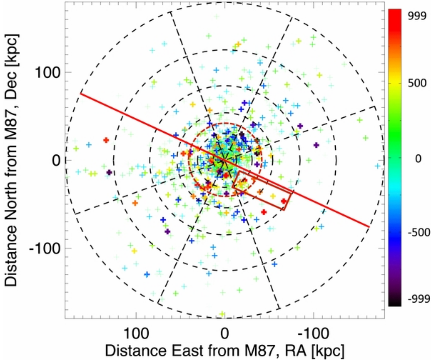
Figure 3. from The Next Generation Virgo Cluster Survey. V. Modeling the Dynamics of M87 with the Made-to-measure Method Zhu et al. 2014 ApJ 792 59 doi:10.1088/0004-637X/792/1/59 https://dx.doi.org/10.1088/0004-637X/792/1/59 © 2014. The American Astronomical Society. All rights reserved.
