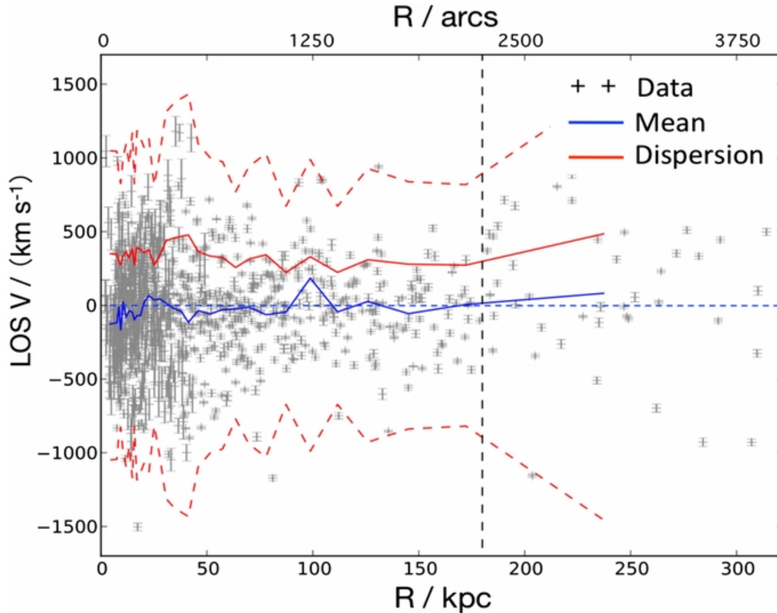
Figure 2. from The Next Generation Virgo Cluster Survey. V. Modeling the Dynamics of M87 with the Made-to-measure Method Zhu et al. 2014 ApJ 792 59 doi:10.1088/0004-637X/792/1/59 https://dx.doi.org/10.1088/0004-637X/792/1/59 © 2014. The American Astronomical Society. All rights reserved.
